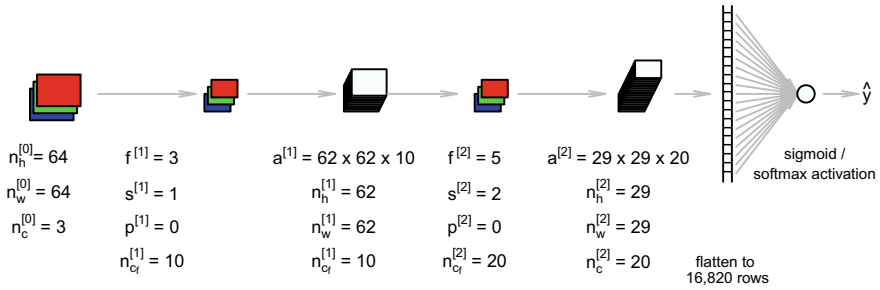
Fig. 7.12 A single-layer Convolution Network diagram
