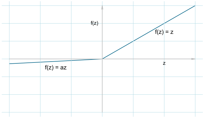
Fig. 2.12 leakyRelu function
