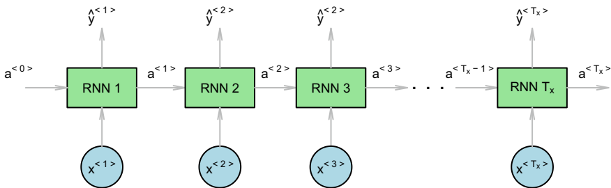
Fig. 8.1 Forward propagation for a basic RNN model
