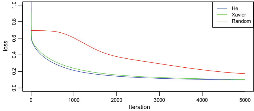
Fig. 4.13 Convergence pattern of different initialization methods
