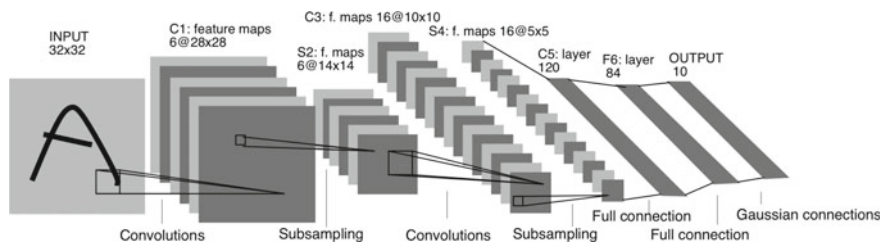
Fig. 7.17 LeNet-5 architecture [21]
