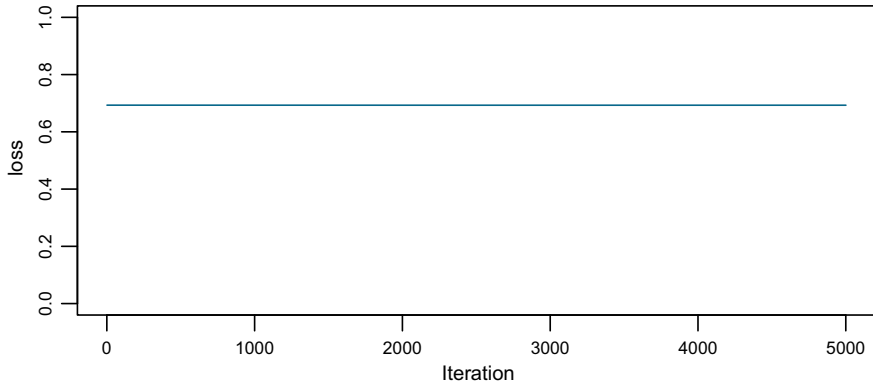
Fig. 4.5 Zero initialization: loss versus iteration
