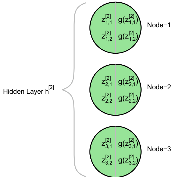
Fig. 2.6 Input and activations represented in the nodes of hidden layer 2
