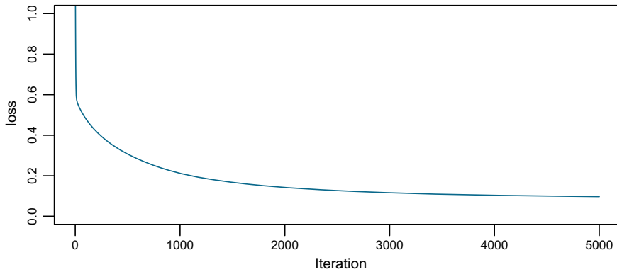
Fig. 4.11 He initialization loss: versus iteration
