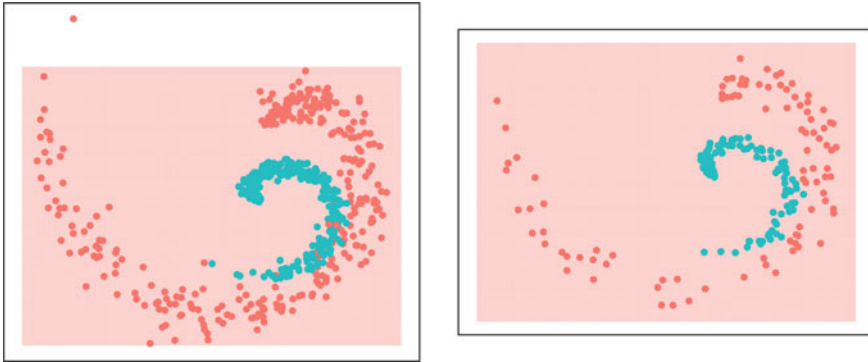
Fig. 4.6 Decision boundary with zero initialization on the training data set (left-hand plot) and the testing data set (right-hand plot)
