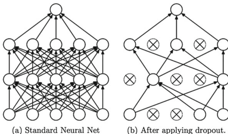
Fig. 5.9 Left: A two layer network. Right: Same network with dropout. Crossed units have been dropped [20]
