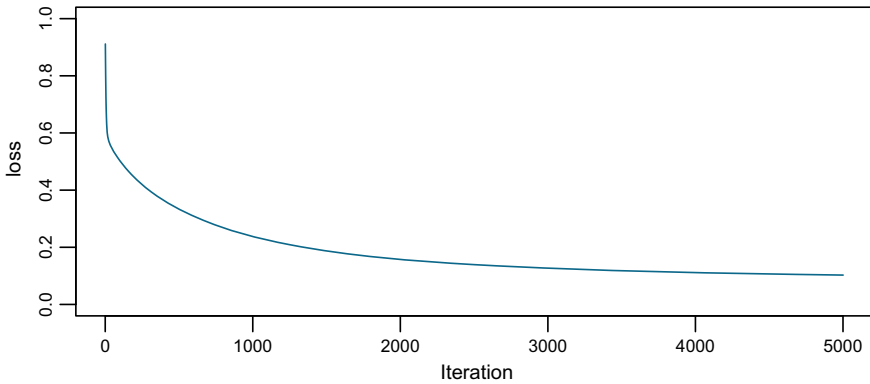
Fig. 4.9 Xavier initialization: loss versus iteration
